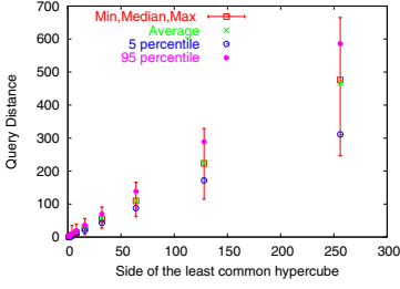
Fig. 5. Query distance vs. smallest common area size. d=2 , L=8 , uniform
